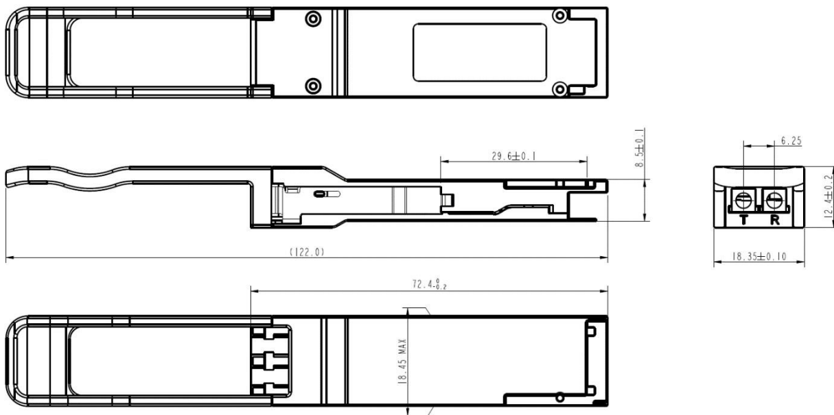
Figure 3. Mechanical Dimensions
