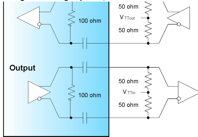
Figure 4-1: High Speed I/O for Data and Clocks
