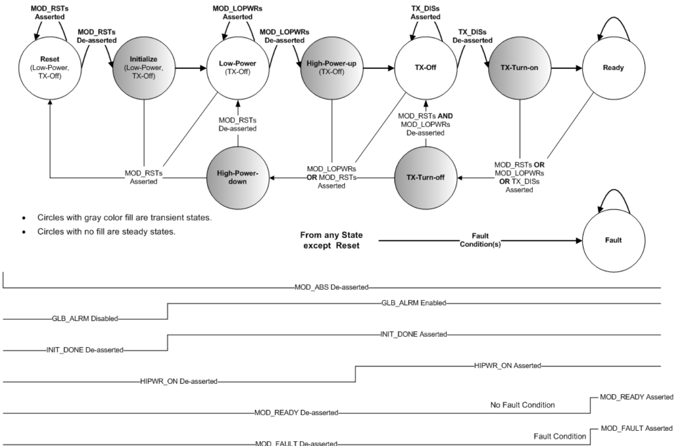
Figure 2-9: CFP MSA Start-Up Flow Diagram
