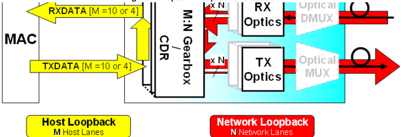
Figure 4-2: Optional Loopback Orientation
