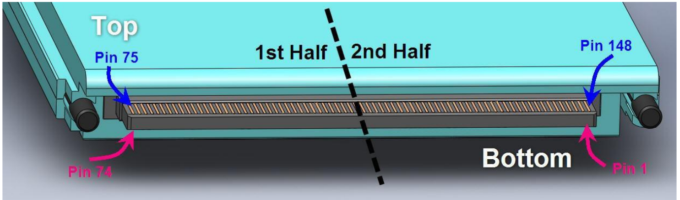
Figure 5-18: CFP Pin Map Orientation
