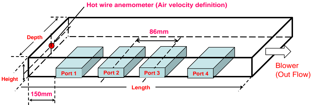
Figure 8-3: Wind tunnel
