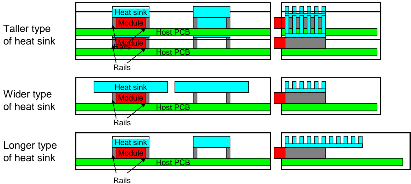
Figure 8-2: Example Riding Heat Sink Configurations
