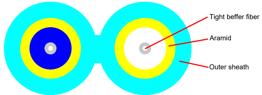
Cable Structure
